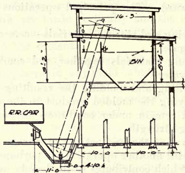
FIG. 17—SUGGESTION FOR ELEVATING EQUIPMENT FOR SAND, GRAVEL AND STONE
